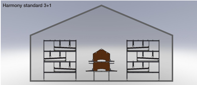
Harmony standard 3+1 Manure belt and perches above nest
